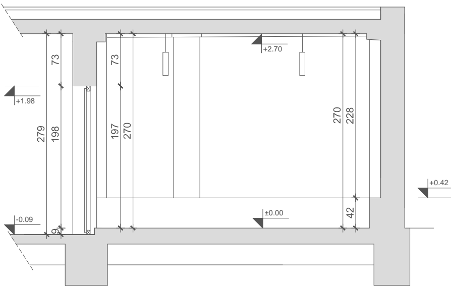
section elevation 3_3
