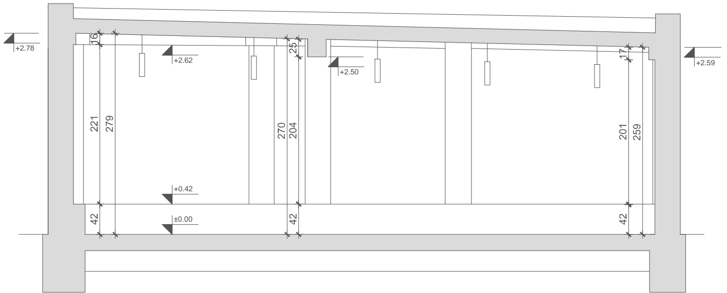
section elevation 1_1
